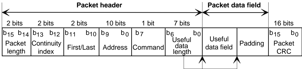
Figure 8: Packet structure
