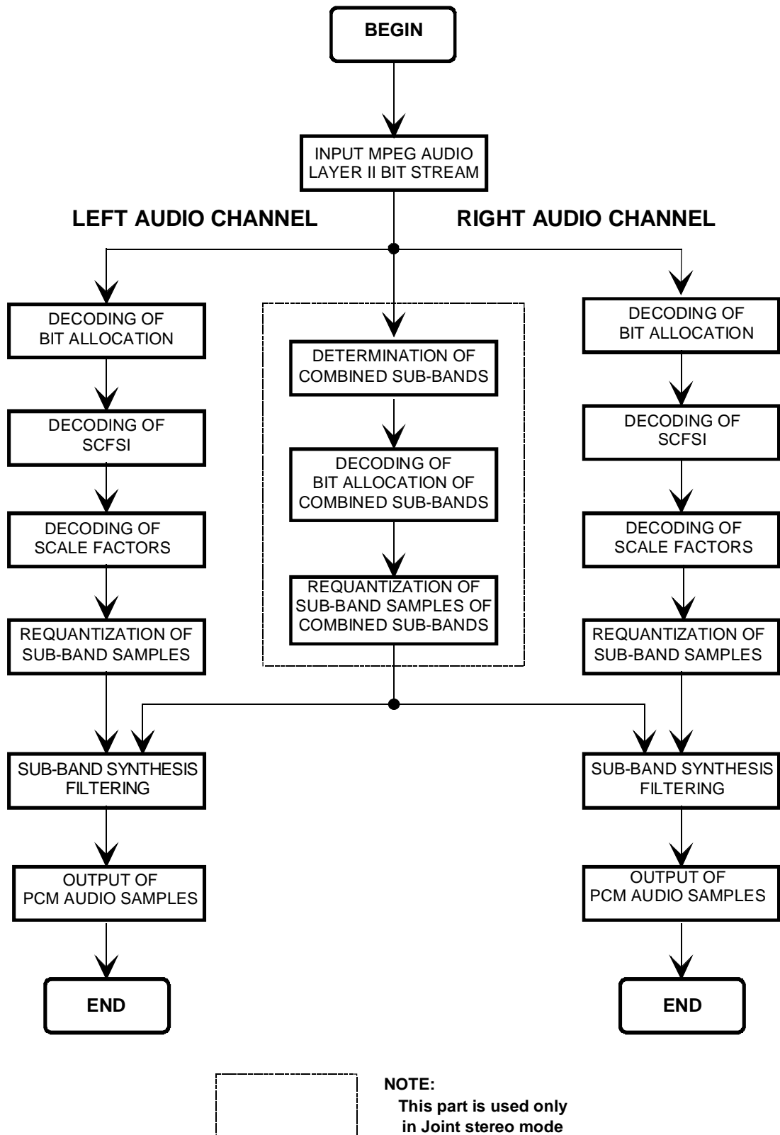
Figure C.3: General MPEG Audio [3, 14] Layer II stereo decoder flow chart
